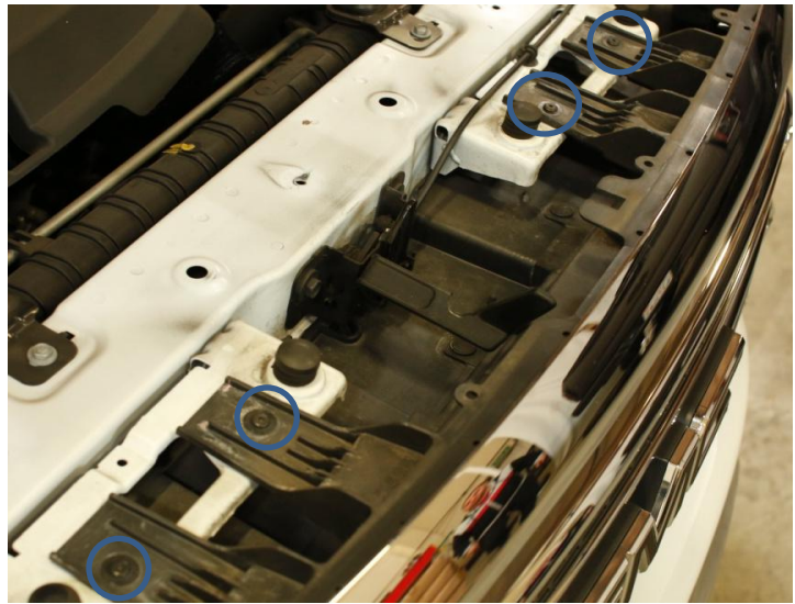
Step 4: Remove four screws with T15 Torx bit to loosen grill.
