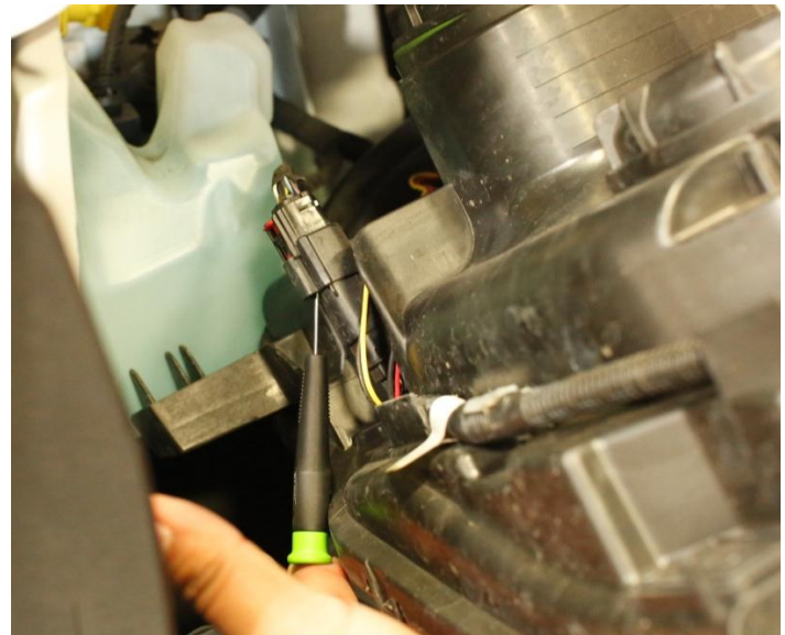
Step 13: Tilt headlight forward to disconnect harness. You might require a small flat head screwdriver to remove connector, then remove headlight.
