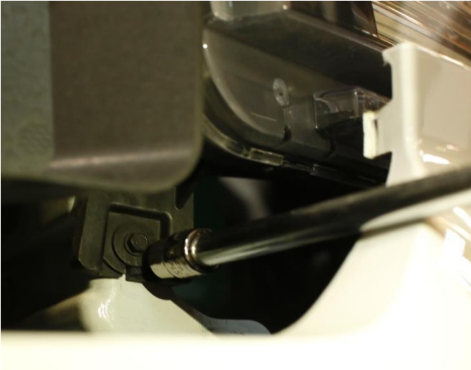
Step 10: Remove OEM headlight by removing four 10mm bolts, one located near radiator.
